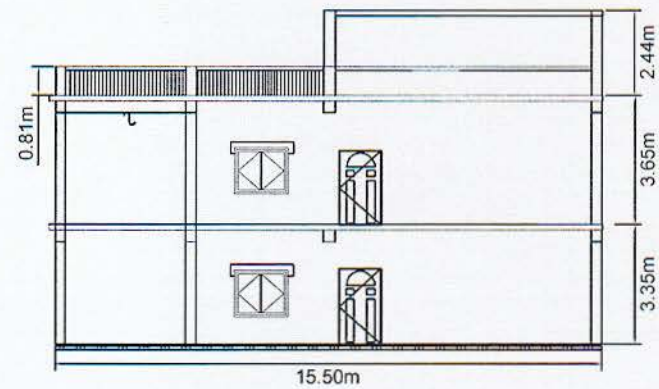
Control Building Front Elevation
