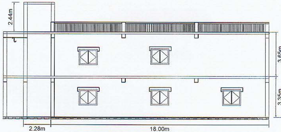
Control Building Right Elevation
