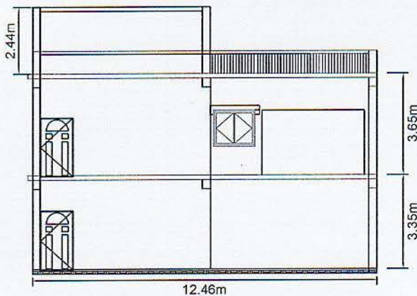
Control Building Front Elevation
