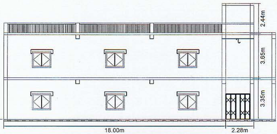
Control Building Left Elevation
