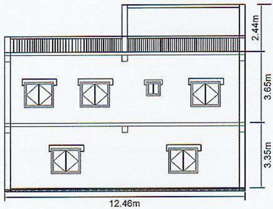
Control Building Back Elevation
