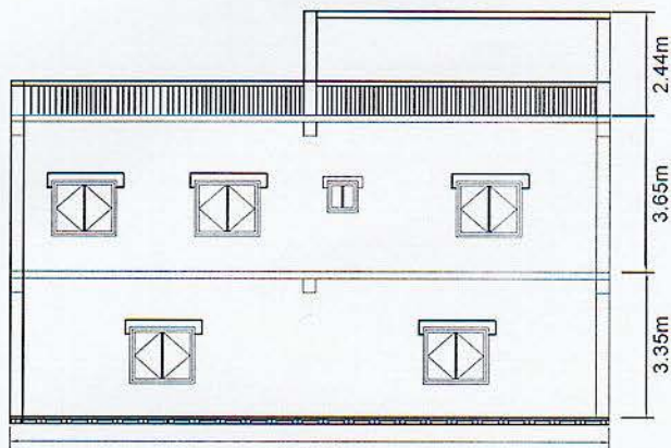
Control Building Back Elevation
