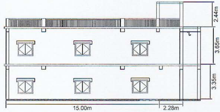
Control Building Left Elevation
