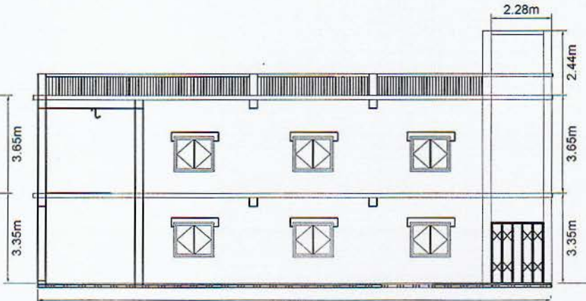
Control Building Left Elevation
