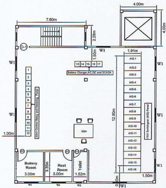
First Floor Plan ( Control Building Plan )
