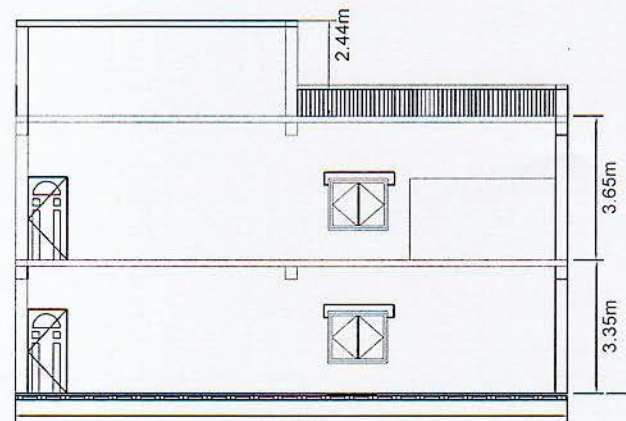
Control Building Front Elevation
