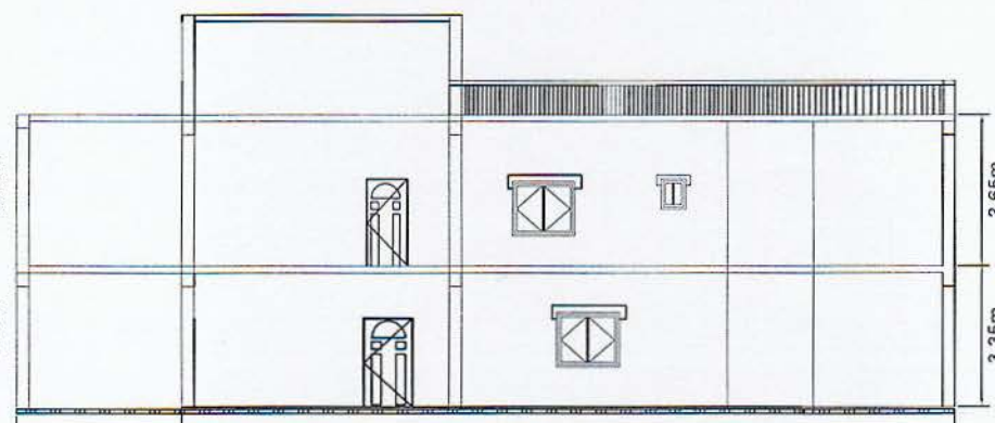
Control Building Front Elevation
