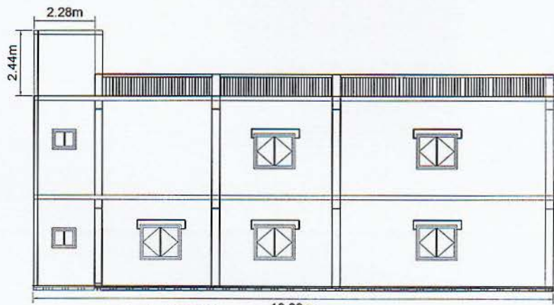
Control Building Right Elevation
