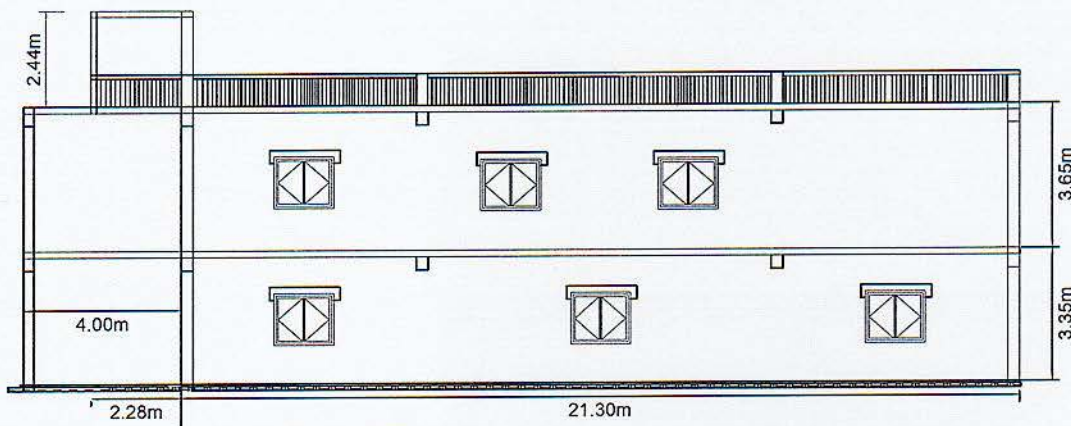
Control Building Right Elevation
