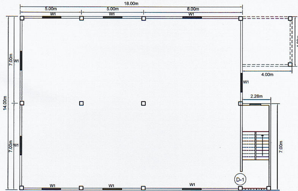
Ground Floor Plan ( Control Building Plan )
