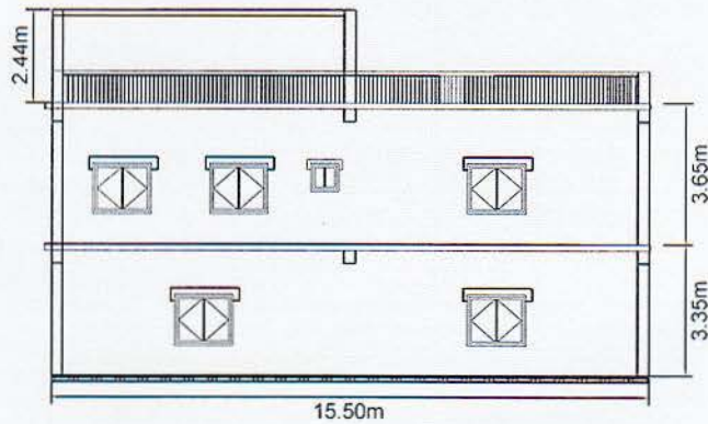
Control Building Back Elevation
