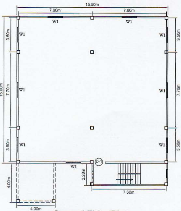
Ground Floor Plan (Control Building Plan)
