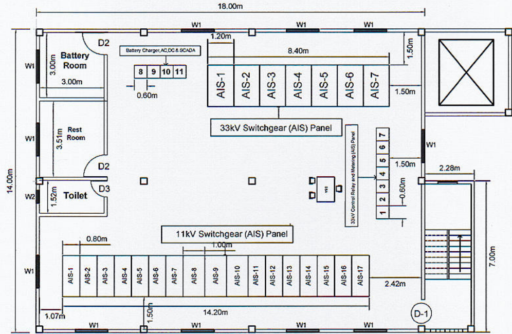
First Floor Plan ( Control Building Plan )
