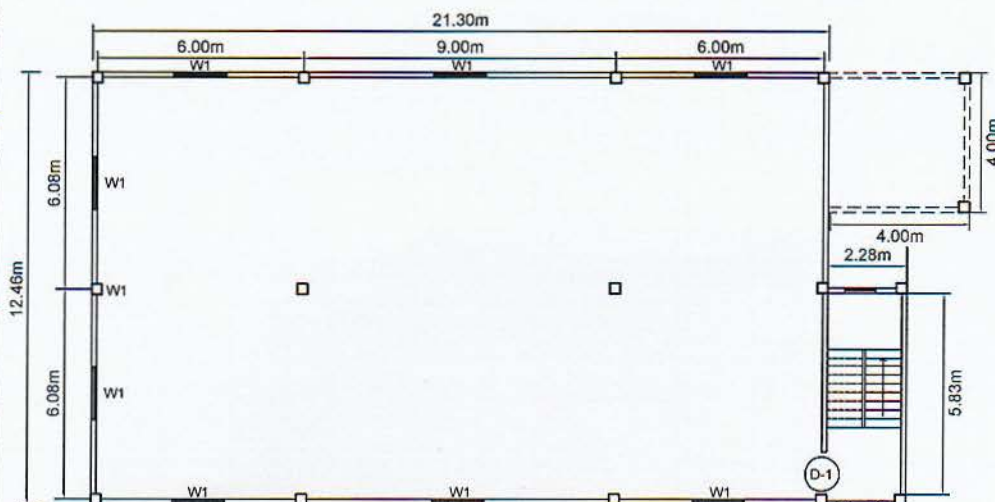
Ground Floor Plan ( Control Building Plan )
