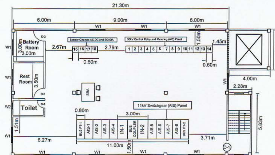
First Floor Plan ( Control Building Plan )
