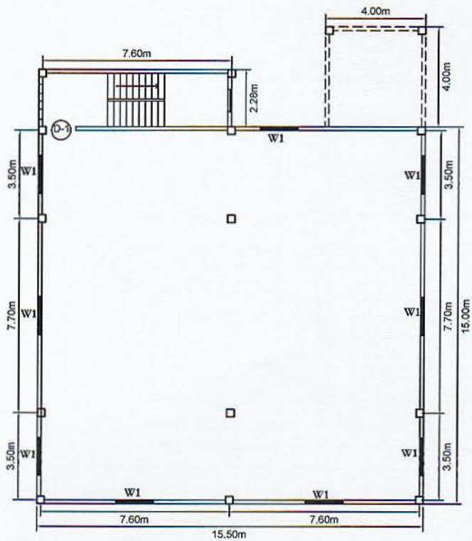
Ground Floor Plan ( Control Building Plan )
